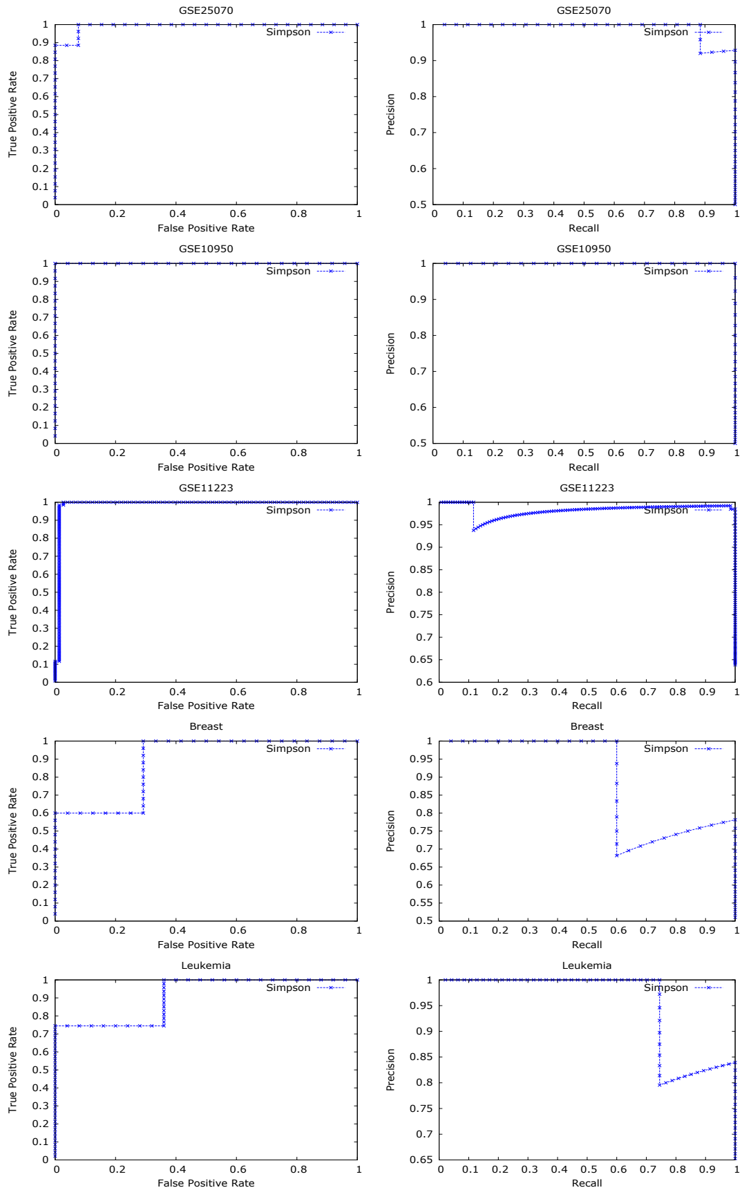
Fig. 7. AUC and AUPR graphs for different data sets using Simpson
