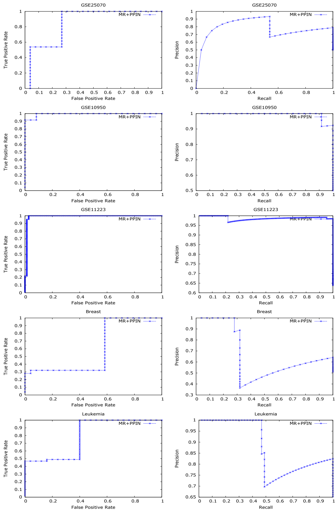
Fig. 1. AUC and AUPR graphs for different data sets using the MR+PPIN method
