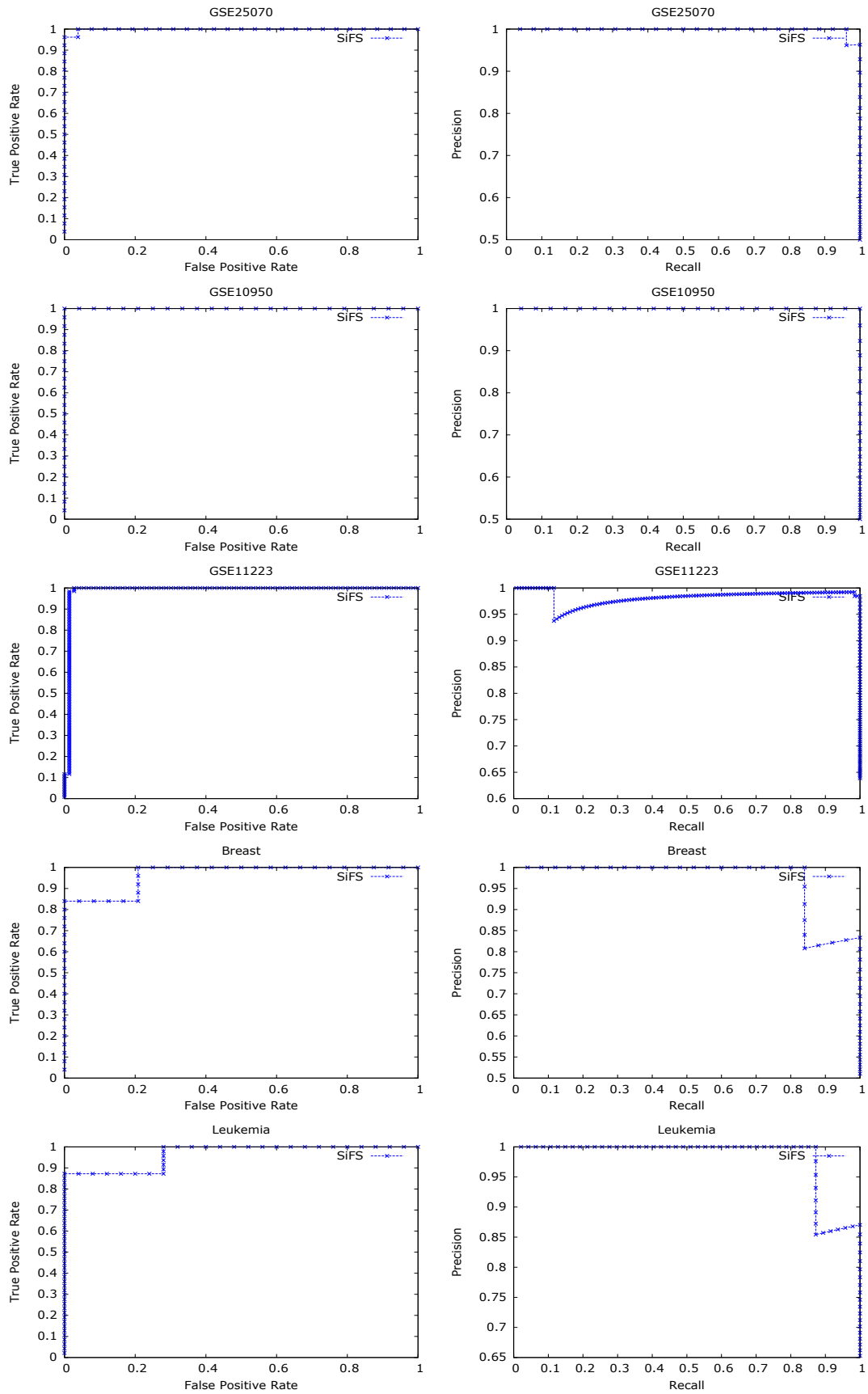
Fig. 5. AUC and AUPR graphs for different data sets using the Cosine-based SiFS method
