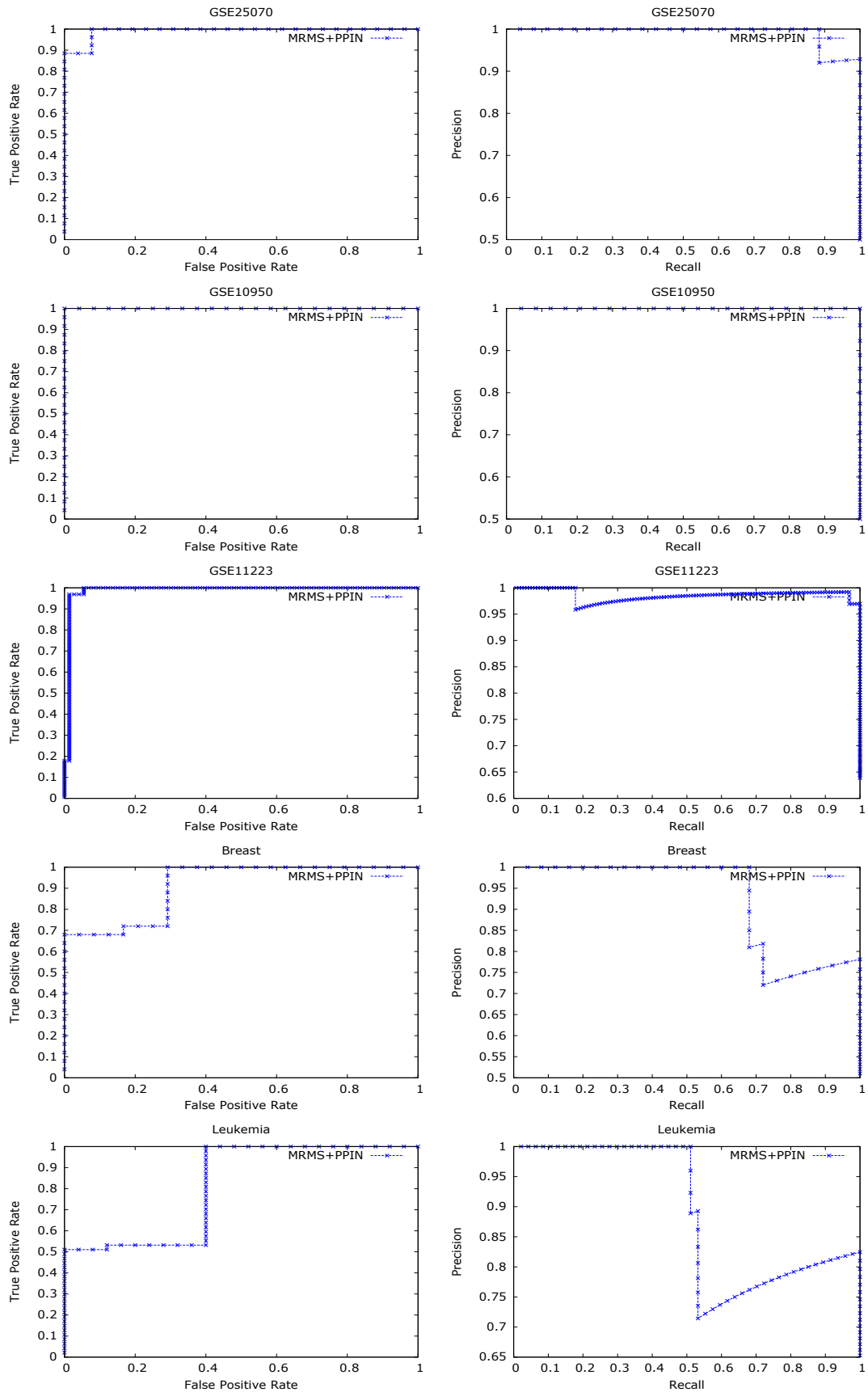
Fig. 3. AUC and AUPR graphs for different data sets using the MRMS+PPIN method
