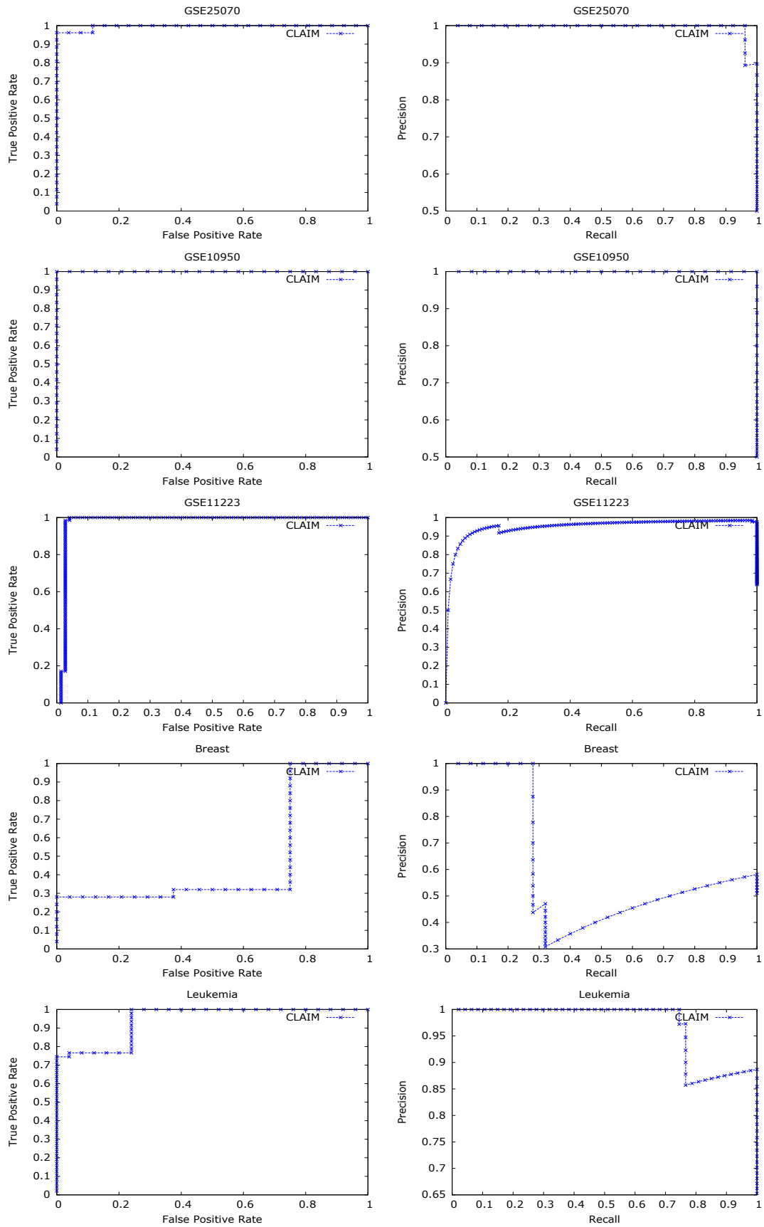
Fig. 4. AUC and AUPR graphs for different data sets using CLAIM
