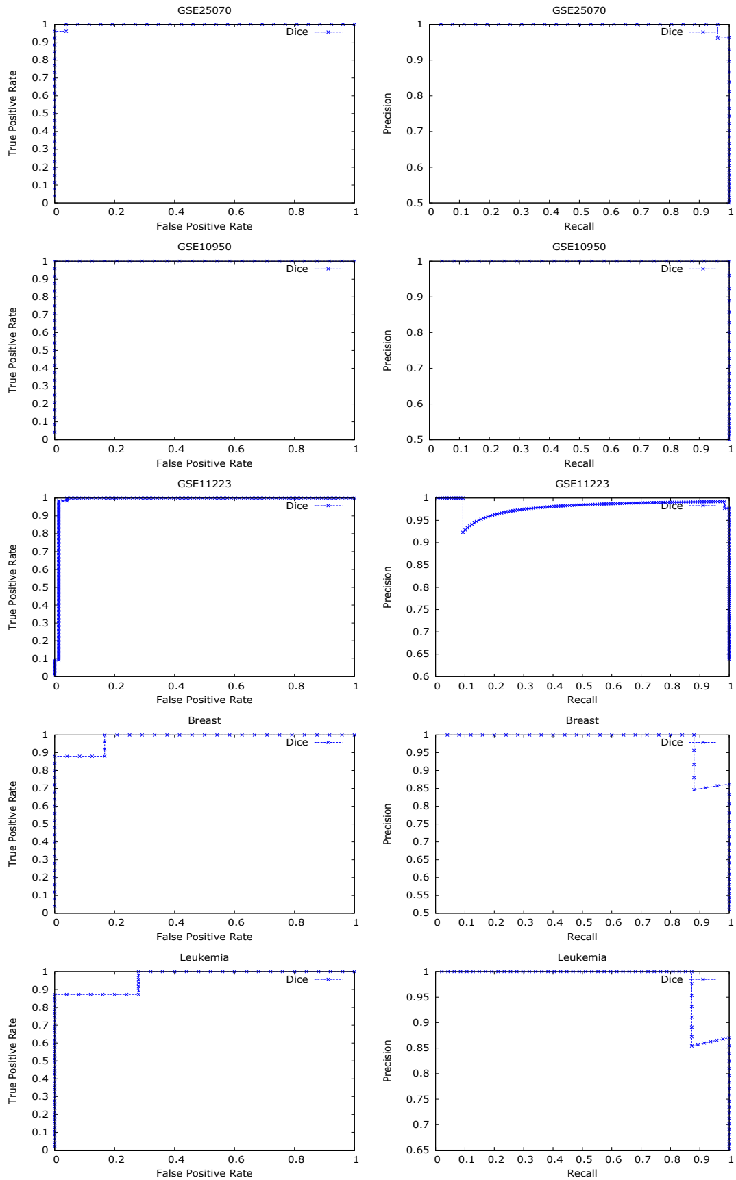
Fig. 9. AUC and AUPR graphs for different data sets using Dice
