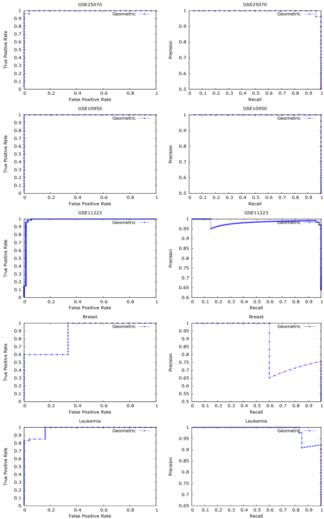
Fig. 8. AUC and AUPR graphs for different data sets using Geometric
