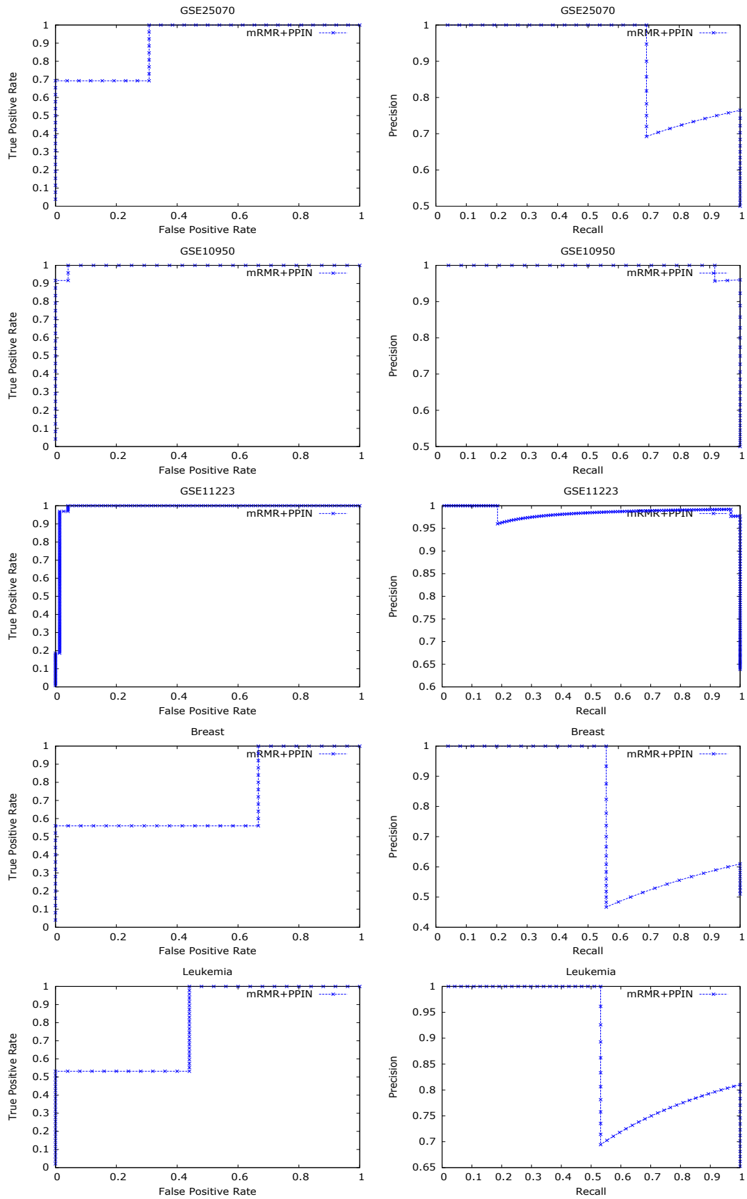
Fig. 2. AUC and AUPR graphs for different data sets using the mRMR+PPIN method
