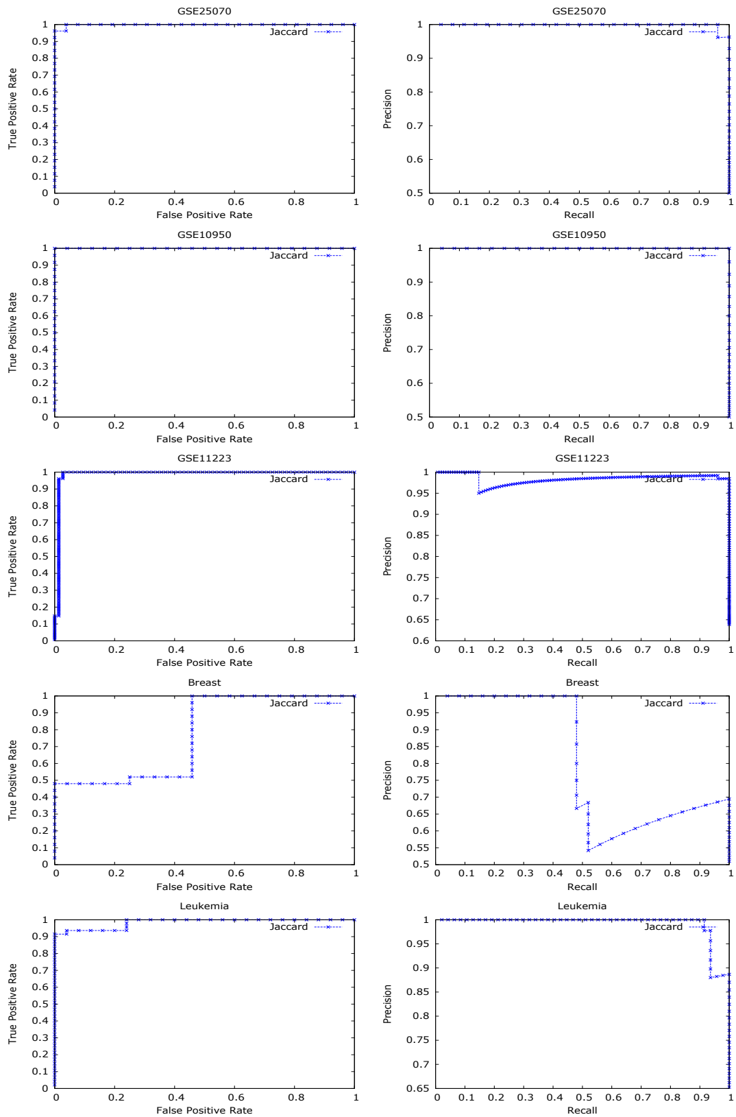
Fig. 6. AUC and AUPR graphs for different data sets using Jaccard
