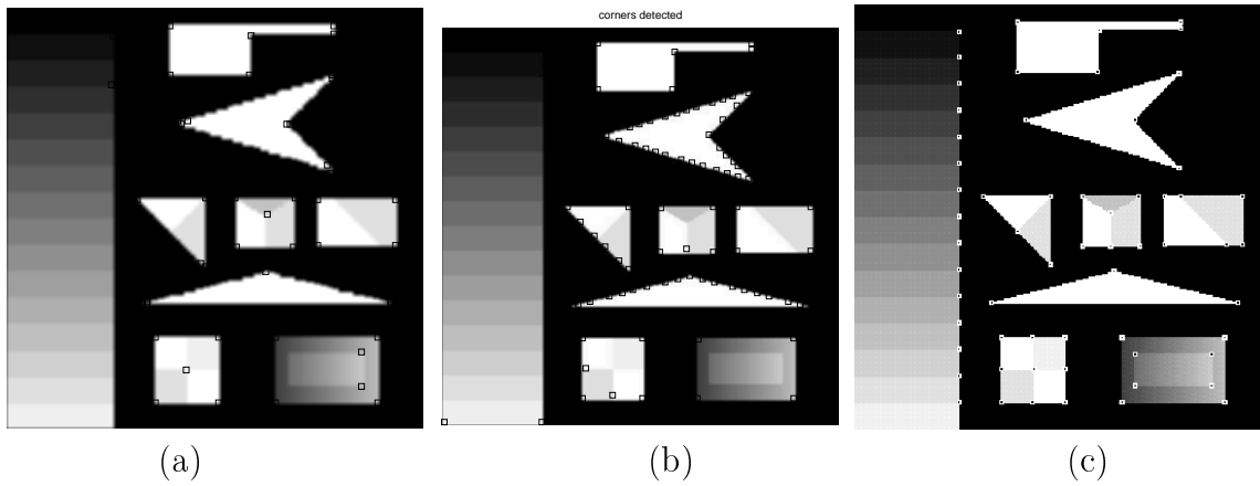
Fig. 15. Corner points (a) Our detector ( \mu_d(P) > 0.0 T_h=0.3 ) (b) Harris detector (c) SUSAN
