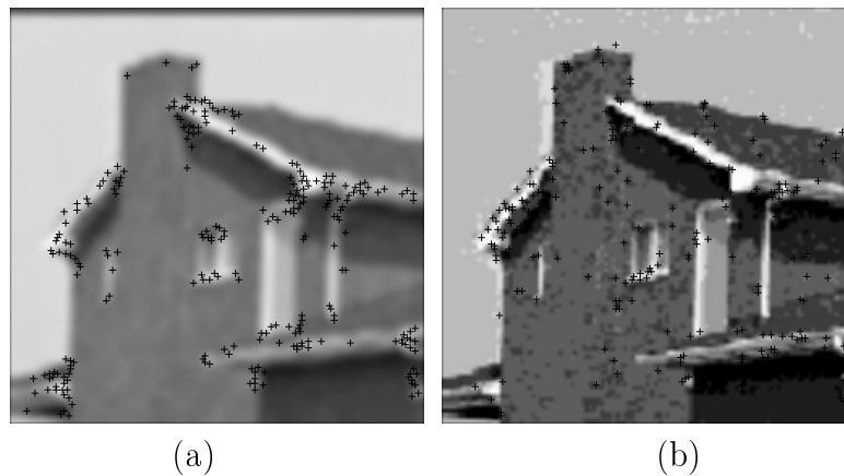
Fig. 17. Corner points from our detector (a) blurred image ( \mu_d(P) \geq 0.9 and T_h=0.2 ) (b) noisy image
