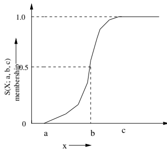
Fig. 1. S-type membership function
