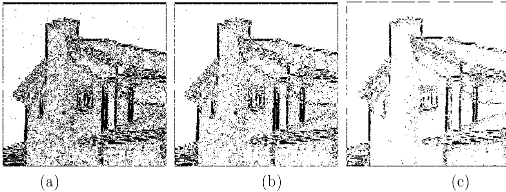
Fig. 7. Fuzzy edge map (a) (\mu_c(P) \geq 0.4) (b) (\mu_d(P) \geq 0.4) after membership transformation(c) (\mu_d(P) \geq 0.9)
