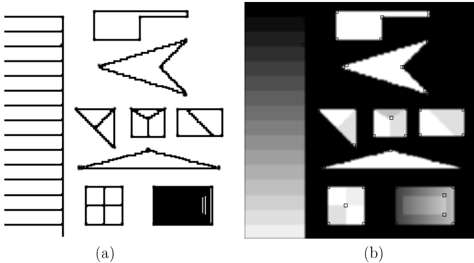
Fig. 13. (a) Curvature points (*), ( \mu_d(P) > 0.0 T_h=0.3 ) (b) Representative points of each cluster
