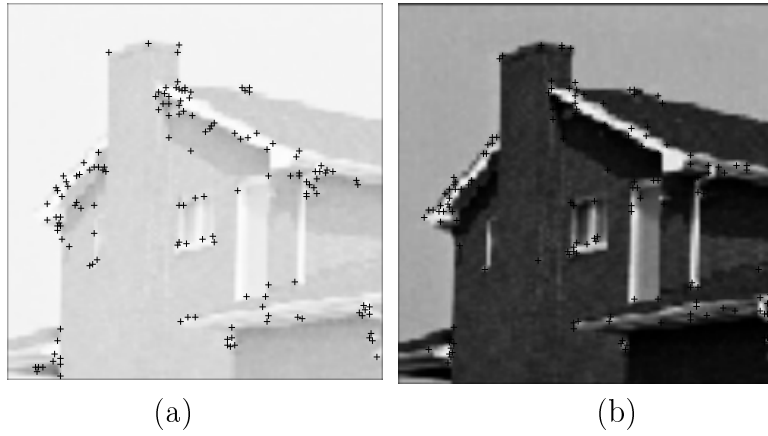
Fig. 18. Corner points under illumination change (a) Overexposed ( \mu_d(P) \geq 0.9 and T_h=0.3 ) (b) Underexposed case ( \mu_d(P) \geq 0.9 and T_h=0.3 )
