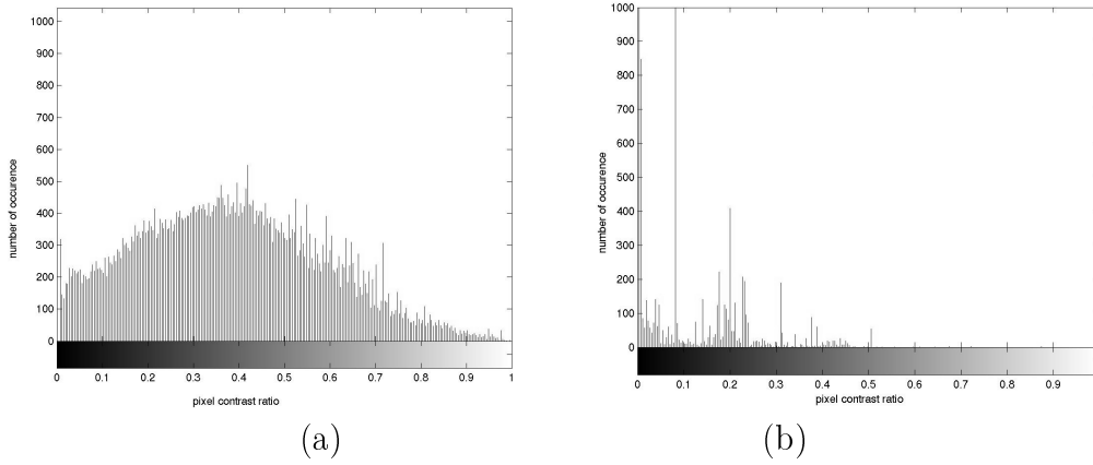
Fig. 6. (a)Pixel contrast histogram of Fig. 5(a) (b)Pixel contrast histogram of Fig. 5(b)
