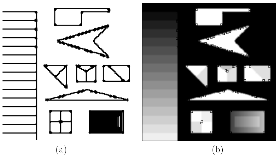
Fig. 14. (a) Curvature points (*), ( \mu_d(P) > 0.6 and T_h = 0.1 ) (b) Representative point of each cluster
