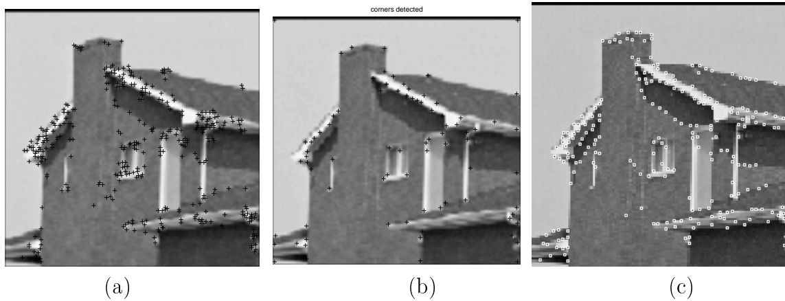
Fig. 16. Corner points (a) Our detector ( \mu_d(P) \geq 0.9 and T_h=0.2 ) (b) Harris detector (c) SUSAN
