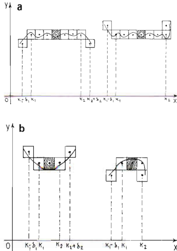
Figure 2. Possible behaviour of f_a(x) when f(x) is constant. (a) Considering local maxima/minima of f_a(x) . (b) Considering global maximum/minimum of f_a(x) . ■ denotes the position of the key pixel.
