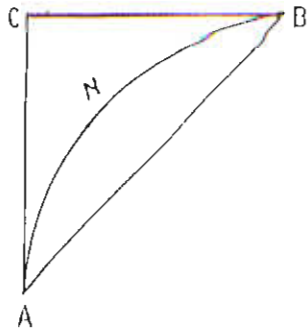
Figure A1. An arc with its associated right triangle.
