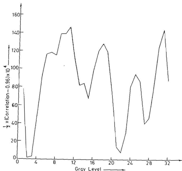
Fig. 4. Curve showing the variation of correlation coefficient with gray levels (using global information) for the image of Lincoln and a window size w of 6.
